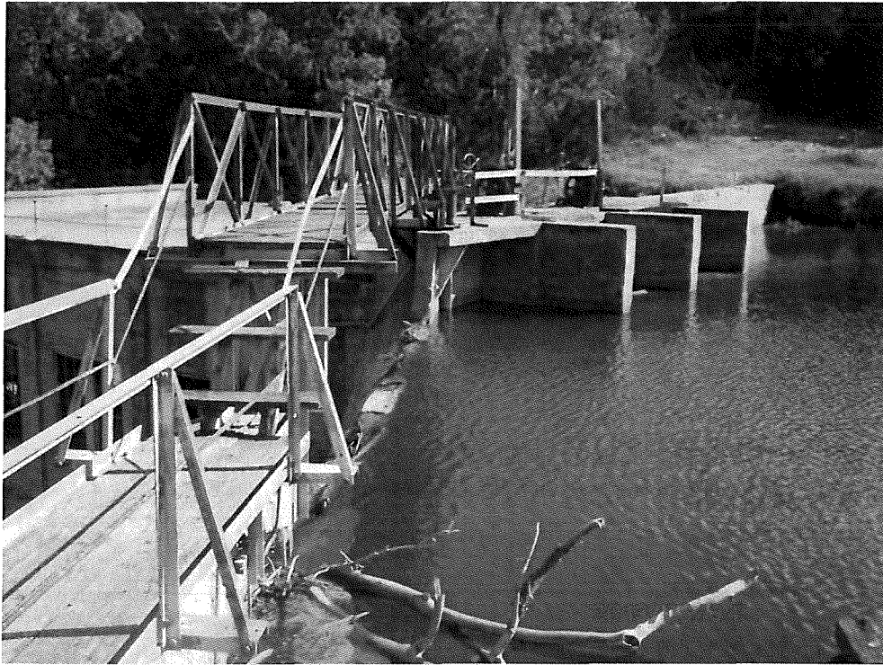
Photo 61 – Spillway catwalk with penstock Inlets in the background, looking to the right abutment.
