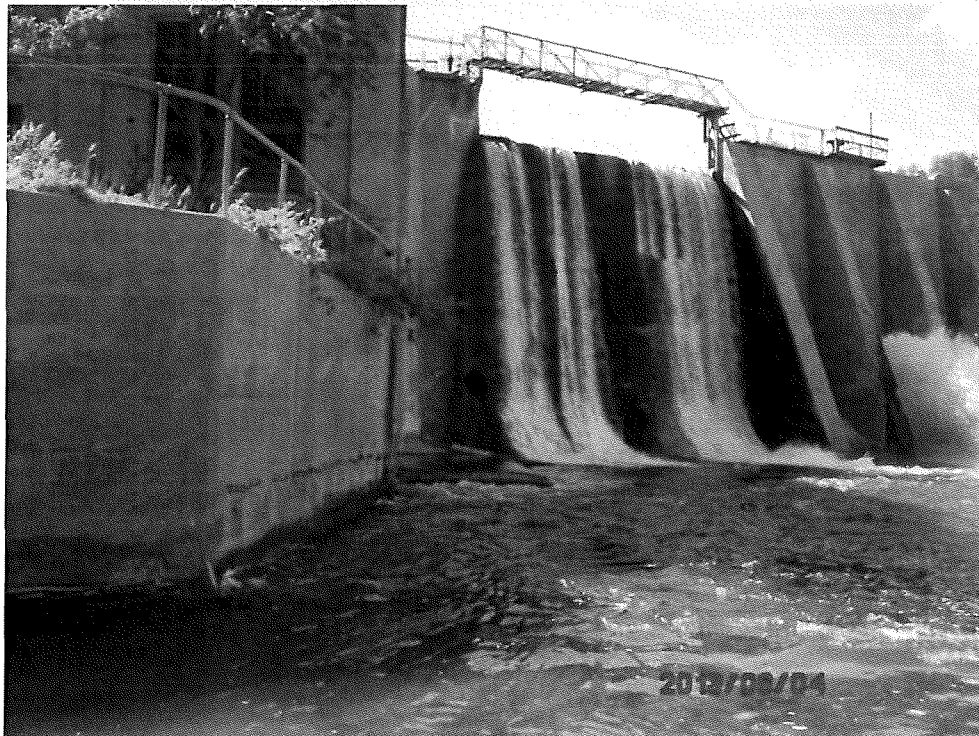
Photo 70 – Powerhouse training wall and tailrace.
